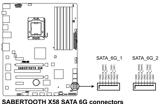
SABERTOOTH X58 SATA 6G connectors
