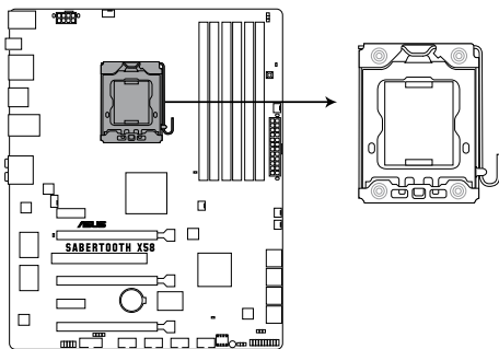
SABERTOOTH X58 CPU LGA1366 socket
