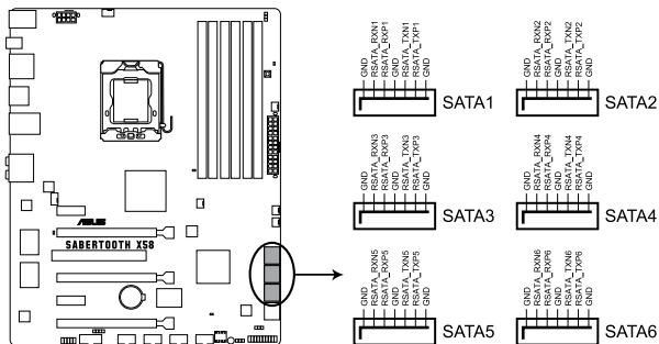
SABERTOOTH X58 SATA connectors
