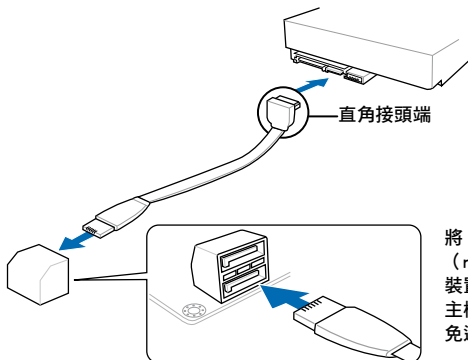
SABERTOOTH X58 SATA connectors
